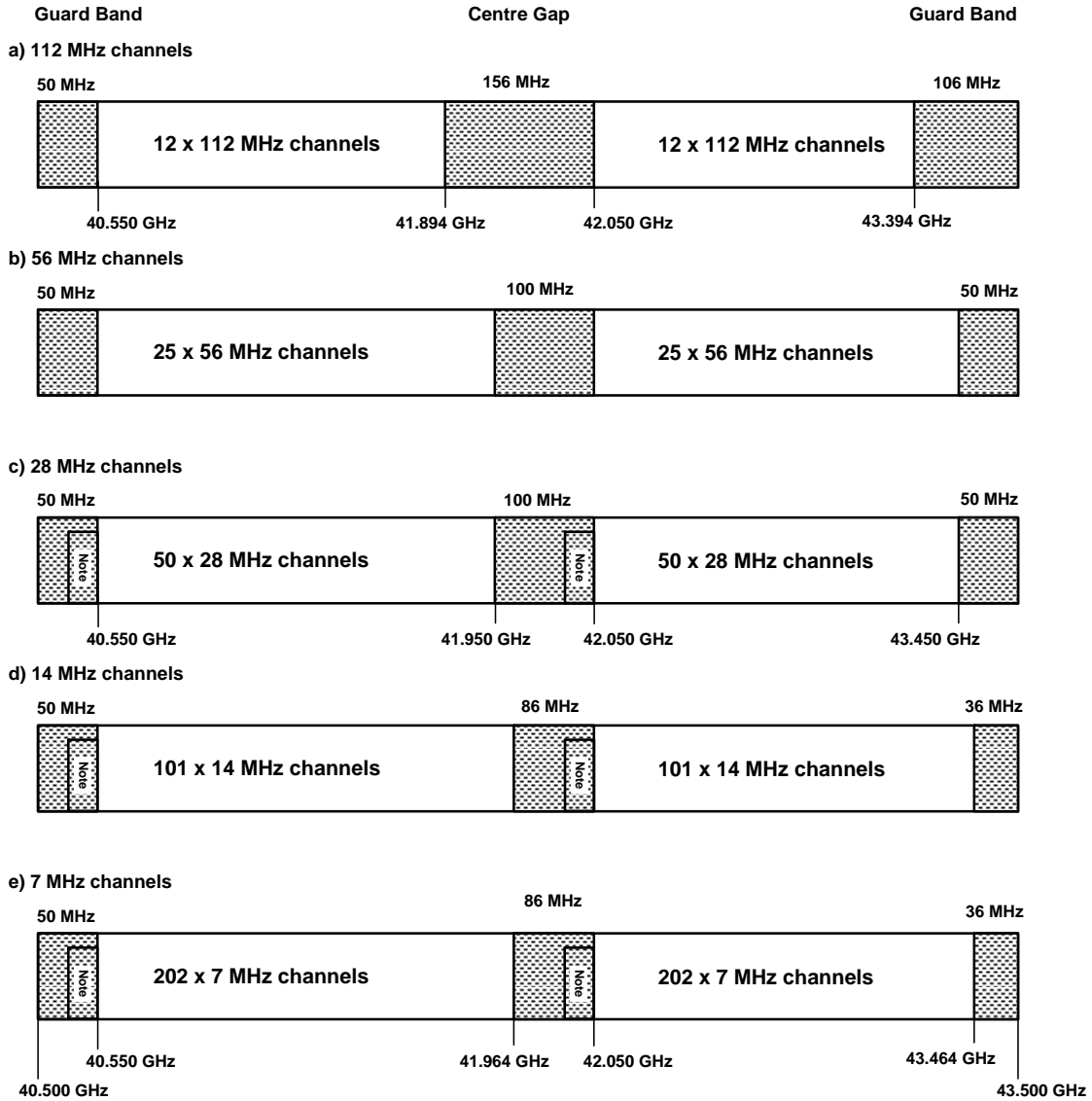
Figure 5.1: Occupied Spectrum from 40.5 to 43.5 GHz
